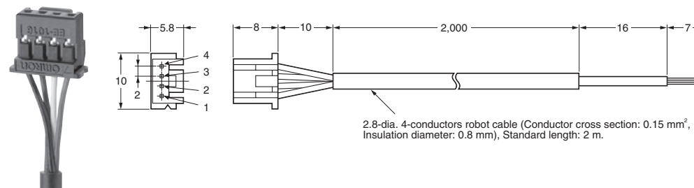
Terminal Arrangement
